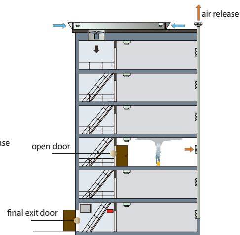
SHAFT AIR RELEASE - PASSIVE
