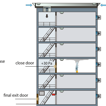
Pressure differential criteria FACADE AIR RELEASE - ACTIVE
