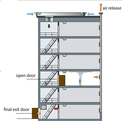
Airflow velocity criteria SHAFT AIR RELEASE - PASSIVE
